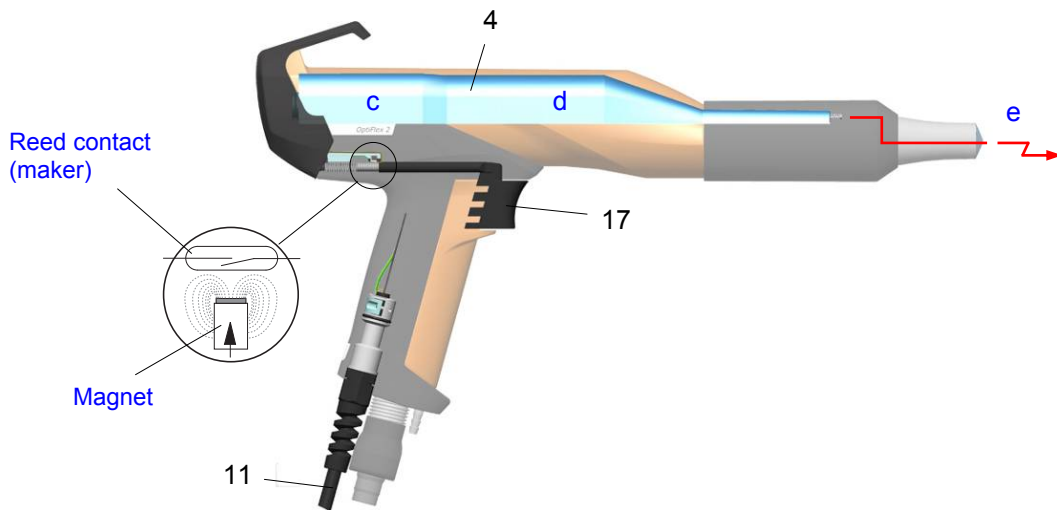
OptiFlex 2 GM03 manual powder gun – Circuitry
